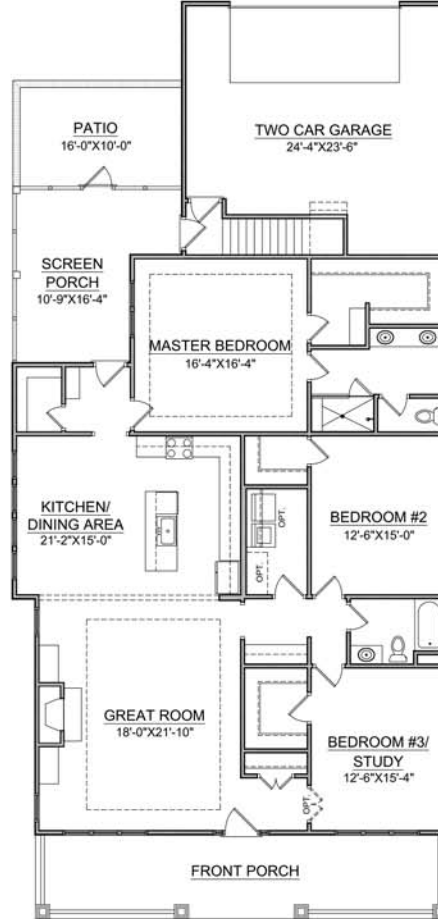
FLOOR PLAN w/ OPT. BONUS ROOM
